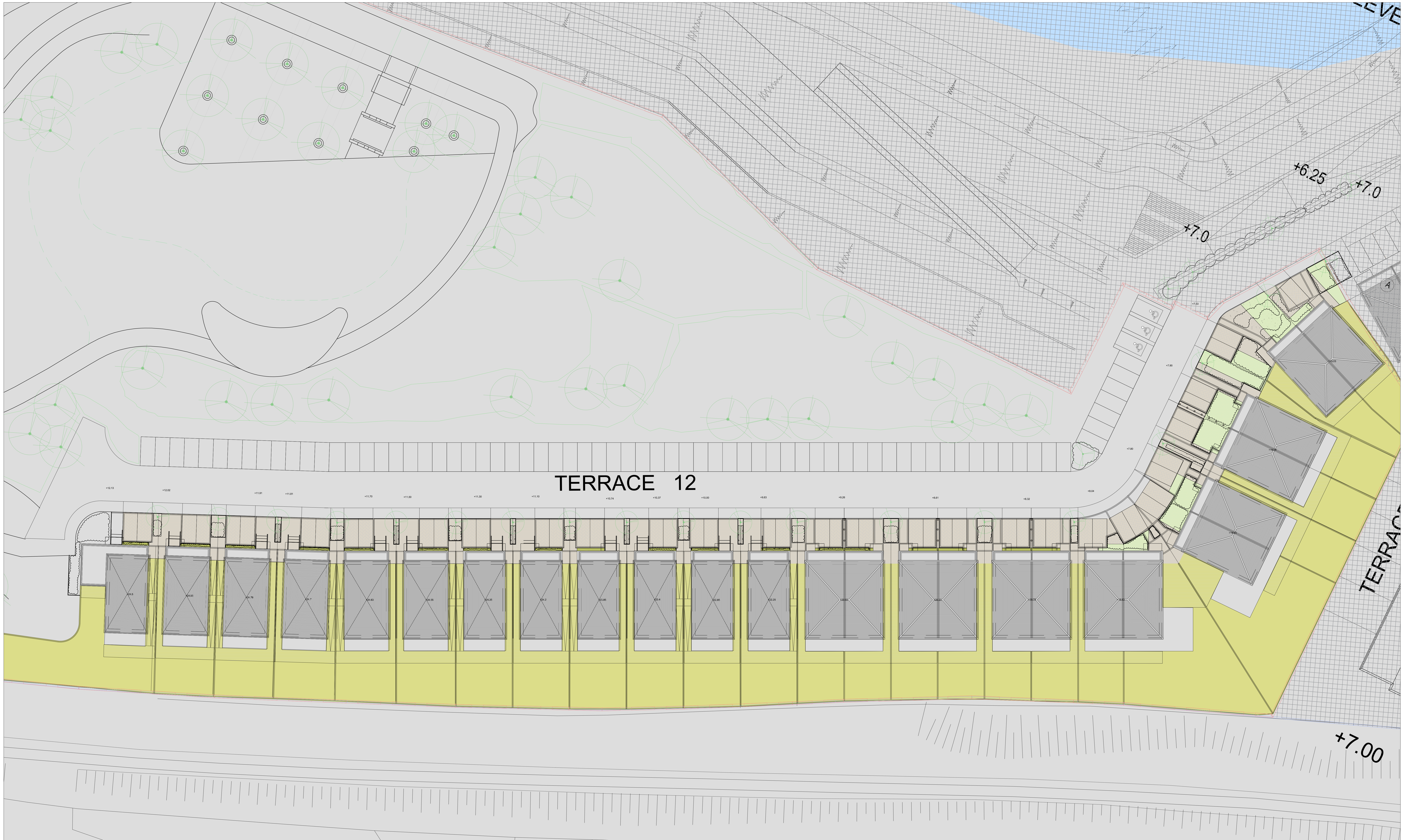
ROOF PLAN SITE LAYOUT_T12 AS PROPOSED
