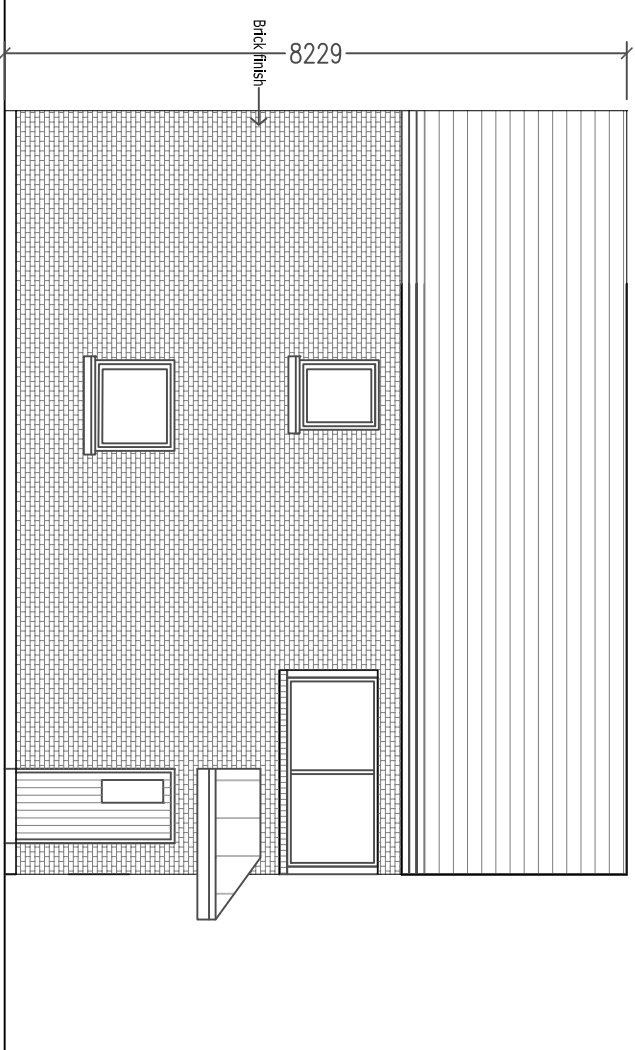
SIDE ELEVATION
