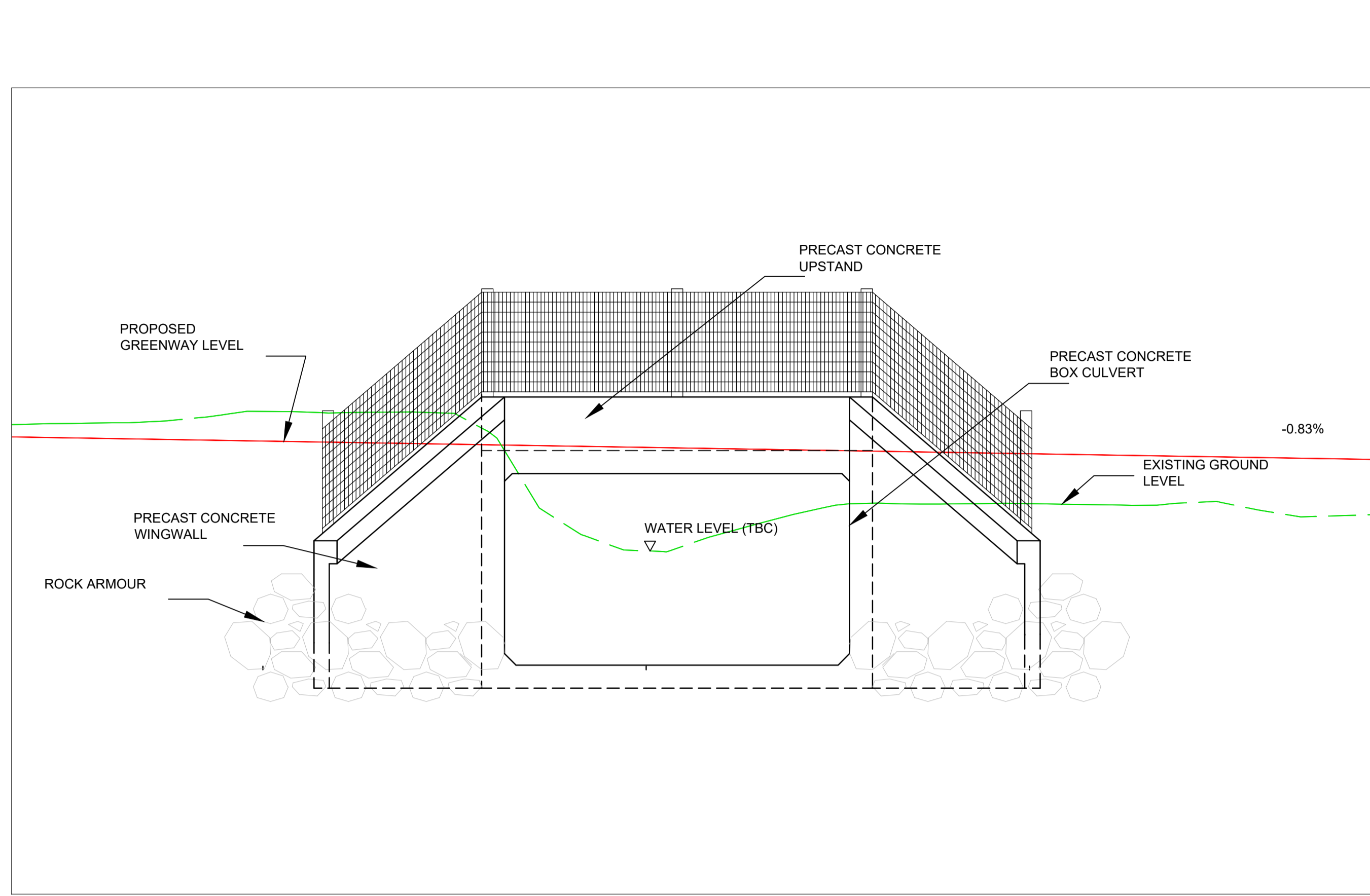
ELEVATION SCALE 1:100
