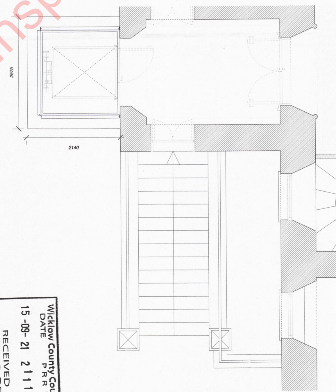
4 FIRST FLOOR PLAN 1:50 @ A2 1:100 @ A4
