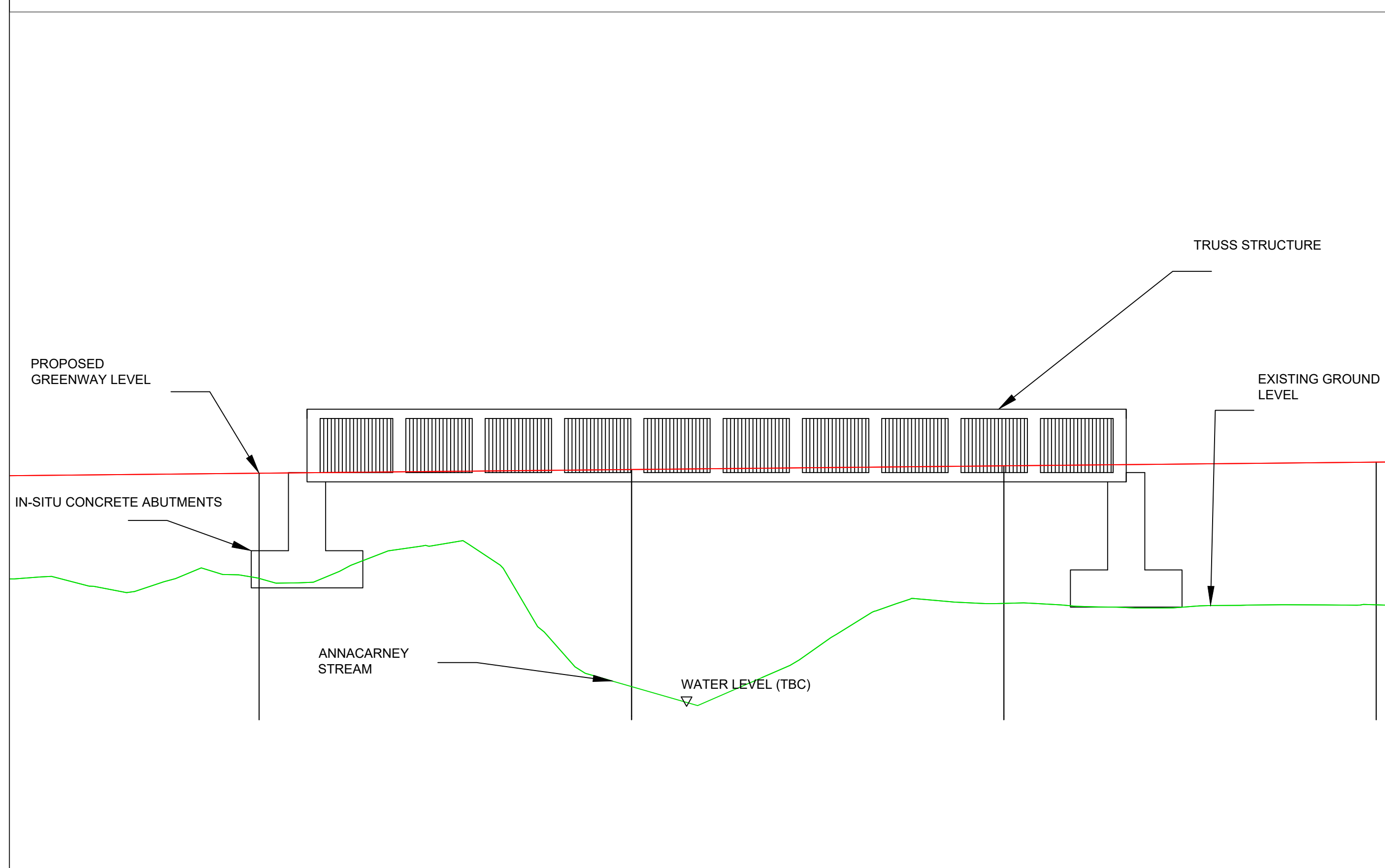
ELEVATION SCALE 1:100
