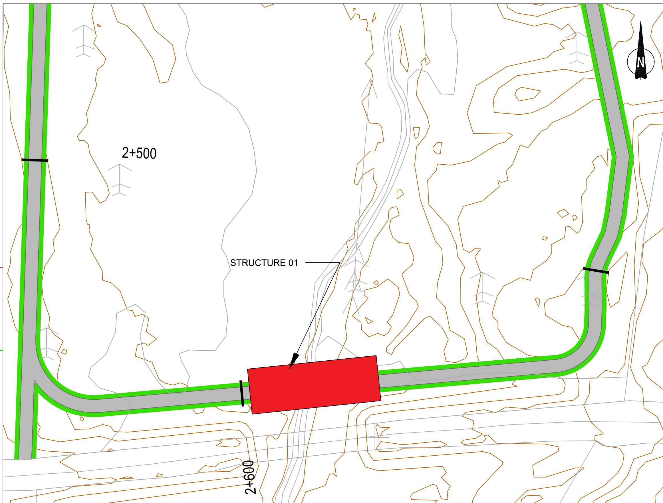
PLAN SCALE 1:500
