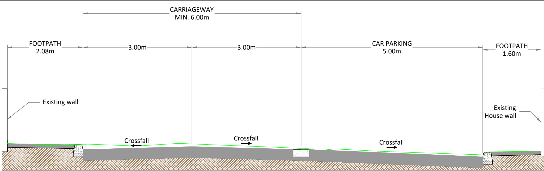
TYPICAL CROSS SECTION C-C SCALE 1:50
