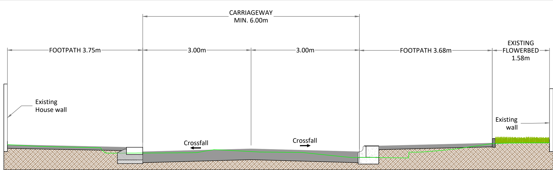
TYPICAL CROSS SECTION D-D SCALE 1:50
